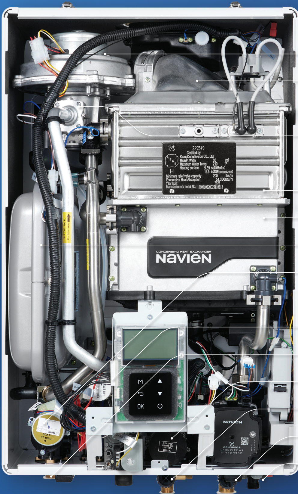
STS Secondary Heat Exchanger
